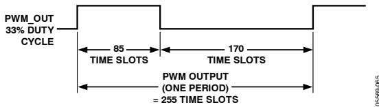
Figure 76. 33% PWM Duty Cycle Represented in Time Slots
