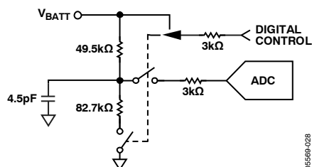
Figure 38. Equivalent V_{BATT} Input Protection Circuit
