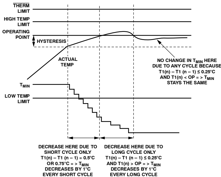
Figure 72. Effect of Exceeding Operating Point Minus Hysteresis Temperature
