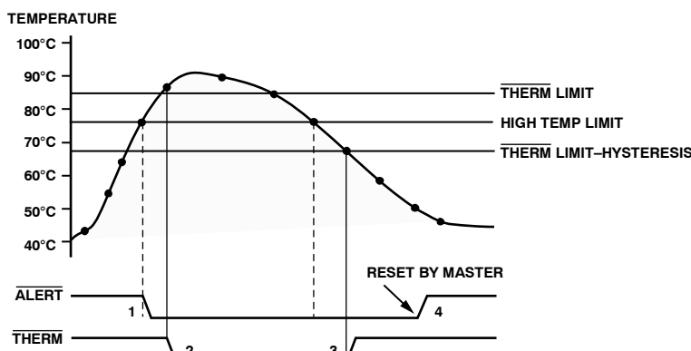
Figure 84. \overline{\text{THERM}} Behavior
