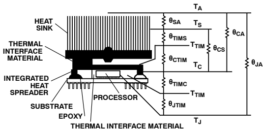
Figure 67. Thermal Model
