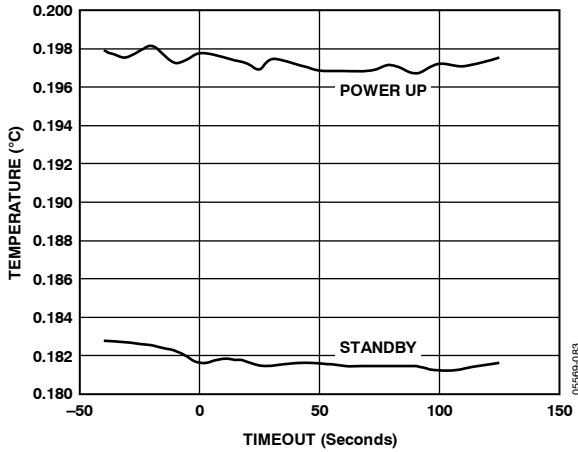
Figure 21. Local Temperature vs. Power-On Reset Timeout
