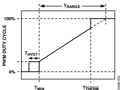
Figure 65. T_{HYST} Value Applies to Fan On/Off Hysteresis
