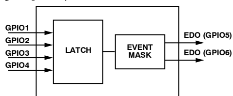
Figure 85. EDO Circuit
