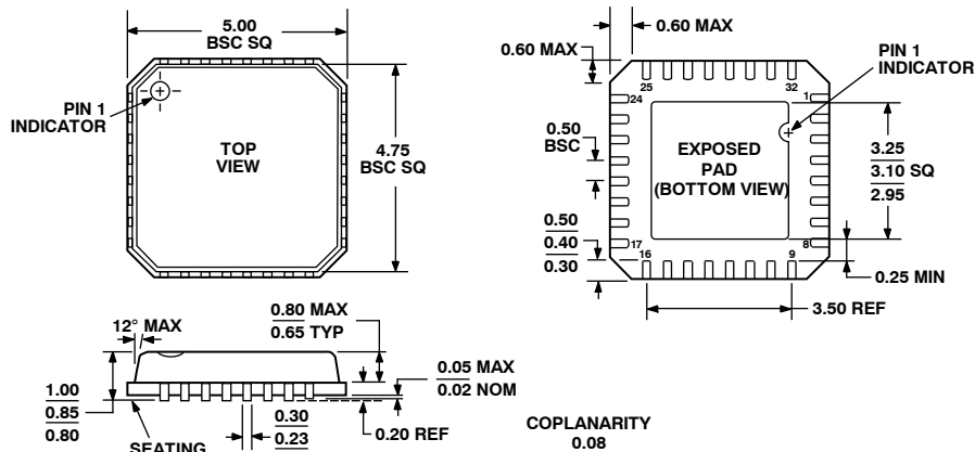
Figure 88. 32-Lead Lead Frame Chip Scale Package [LFCSP_VQ] 5 mm × 5 mm Body, Very Thin Quad (CP-32-2) Dimensions shown in millimeters
