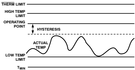
Figure 71. Temperature Between the Operating Point and the Low Temperature Limit
