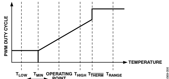
Figure 68. Dynamic T_{MIN} Control Loop
