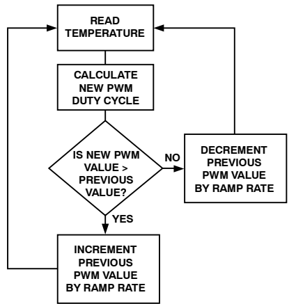
Figure 77. Enhanced Acoustics Mode Algorithm
