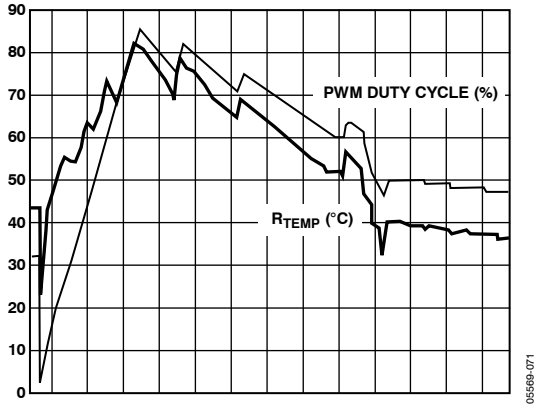
Figure 82. How Fan Reacts to Temperature Variations in Enhanced Acoustics Mode
