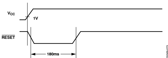
Figure 86. Operation of RESET Output on Power-Up
