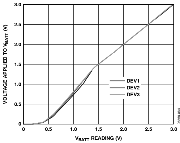
Figure 22. Applied Voltage vs. V_{BATT} Reading
