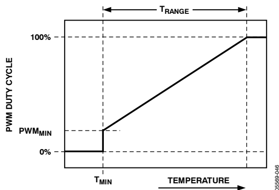
Figure 58. T RANGE Parameter Affects Cooling Range
