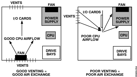
Figure 66. Chassis Airflow Issues
