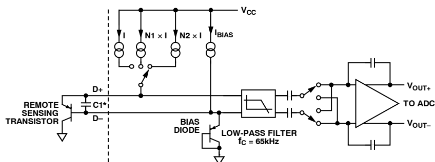
*CAPACITOR C1 IS OPTIONAL. IT SHOULD ONLY BE USED IN NOISY ENVIRONMENTS.
